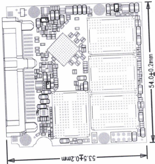
Figure 1-2.5" SATAIII SSD Outline Drawing.
